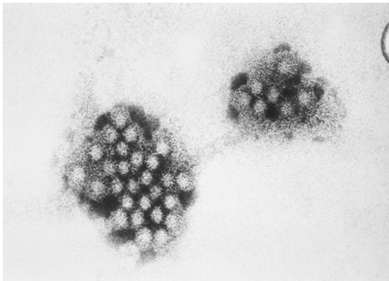
Figure 1 : Norovirus ( Caliciviridae )
